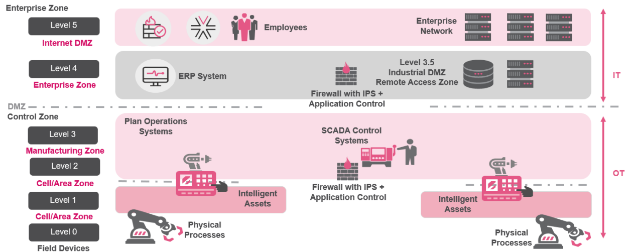
Figure 3: The Purdue Model
