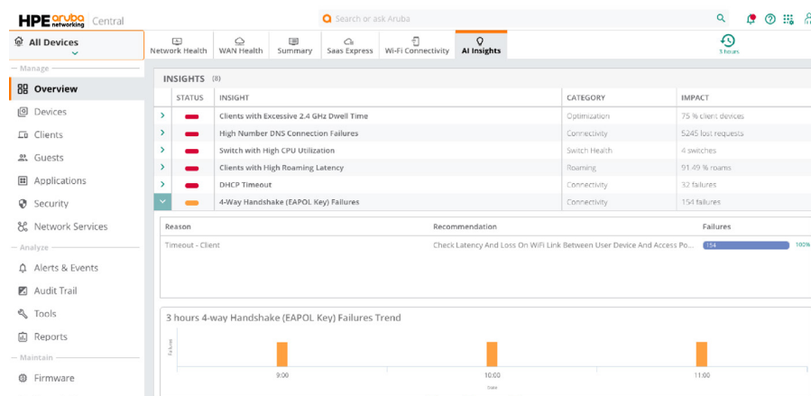
Figure 1. HPE Aruba Networking Network Insights: automated root cause analysis
